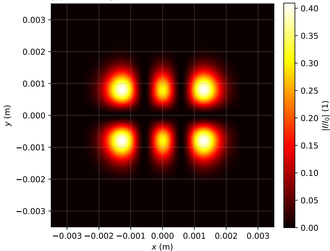
Intensity profile I(x, y, z = 2.548)/I_0 , P_{in}=0.5P_{cr} , artificial time
